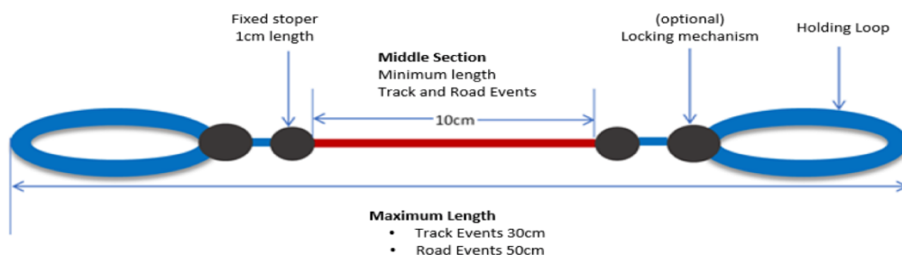
Figure 3 – Tether features
