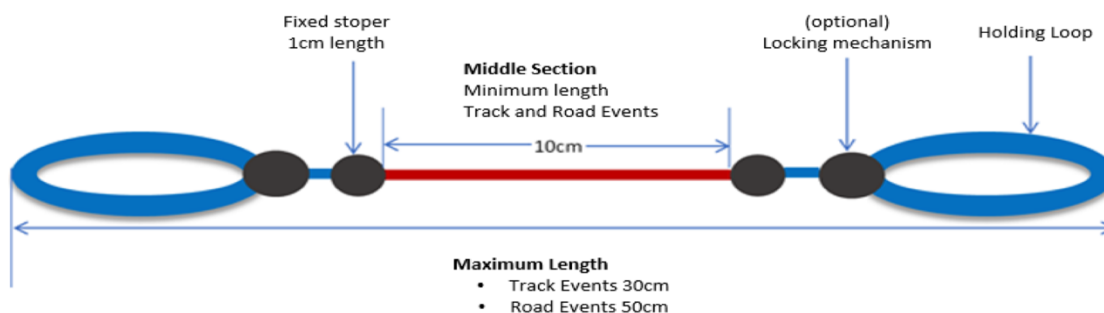
Figure 3 – Tether features
